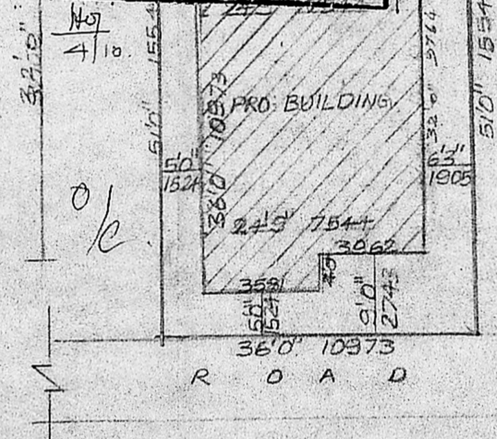
SITE PLAN SCALE 1"=16'0"
