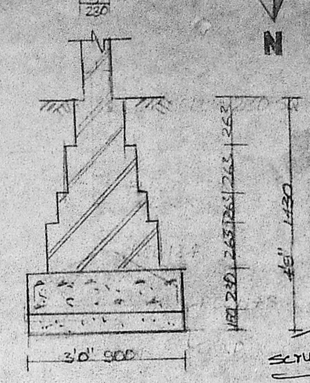
DETAILS OF FOUNDATION
